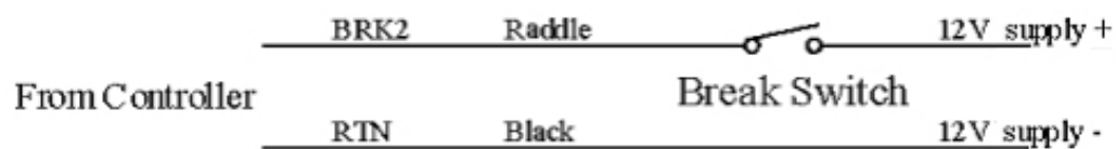
Figure 6: wiring of BRK2
