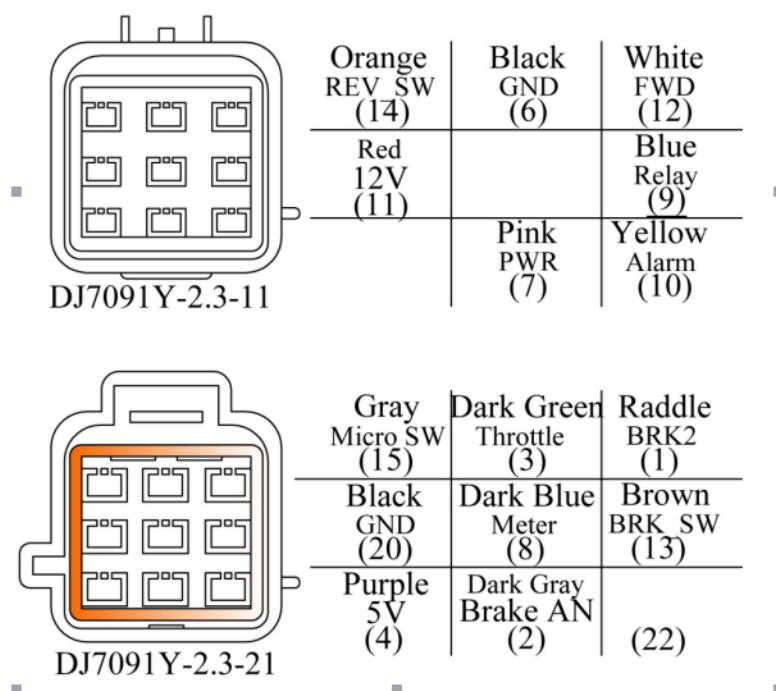
Figure 3: waterproof connector
