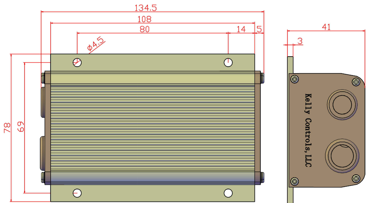
Figure 1:SPM-12S mounting holes' dimensions (dimensions in millimeters)
