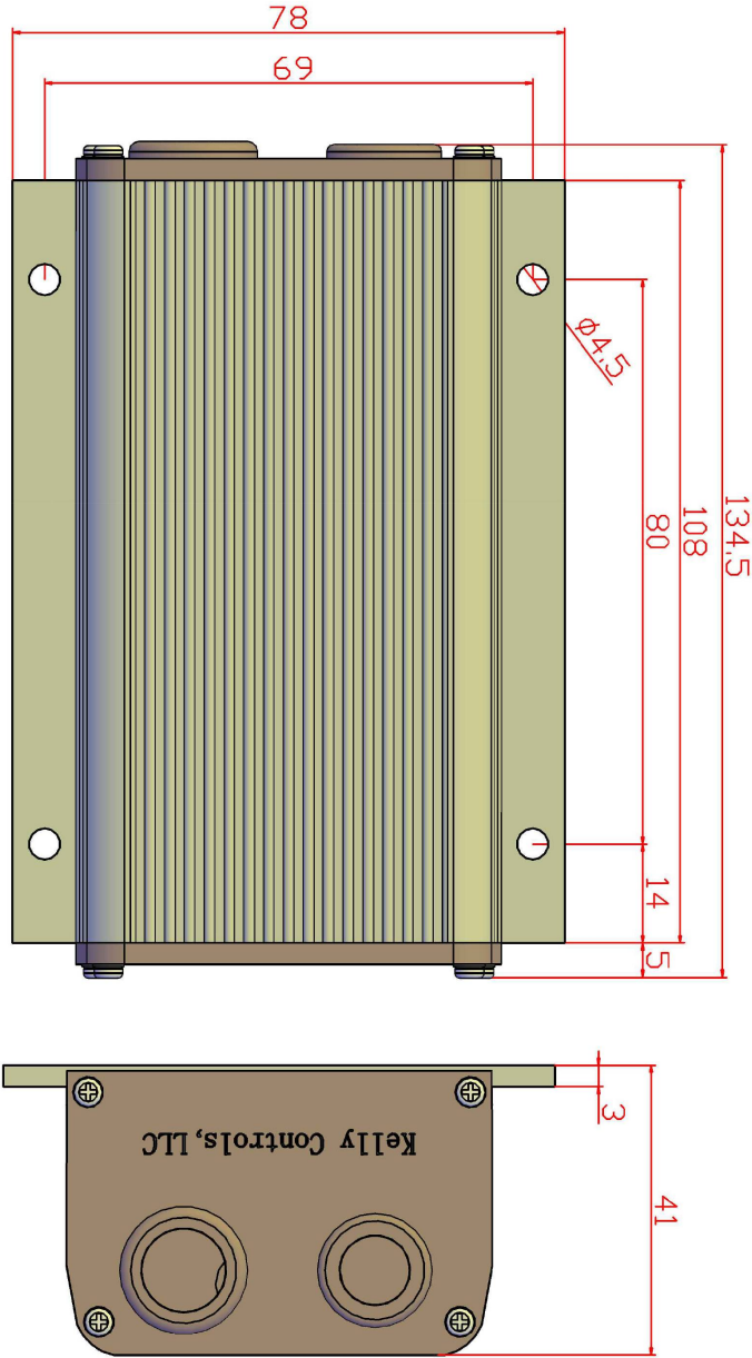
Figure 1:KBS –X mounting holes' dimensions (dimensions in millimeters)
