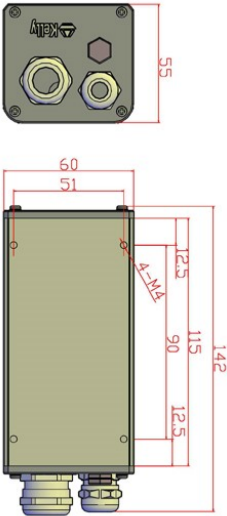
Figure 2: KBS2412Z KBS4812Z KBS7212Z mounting holes' dimensions (dimensions in millimeters)
