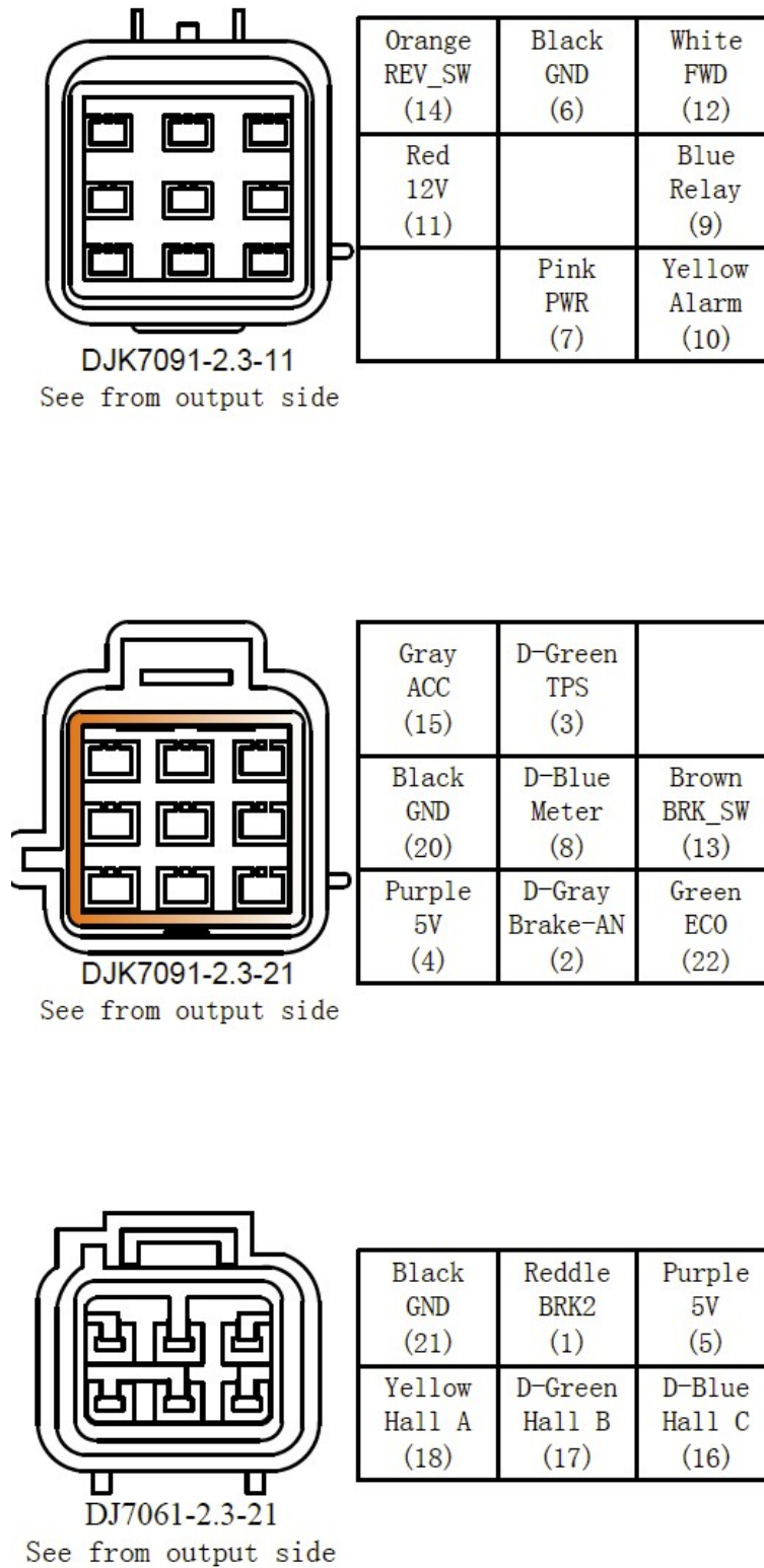
Figure 2: waterproof connector
