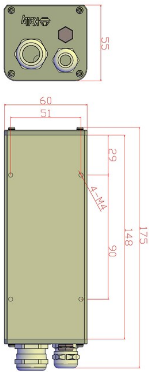
Figure 3: KBS-4818Z KBS7218Z mounting holes' dimensions (dimensions in millimeters)
