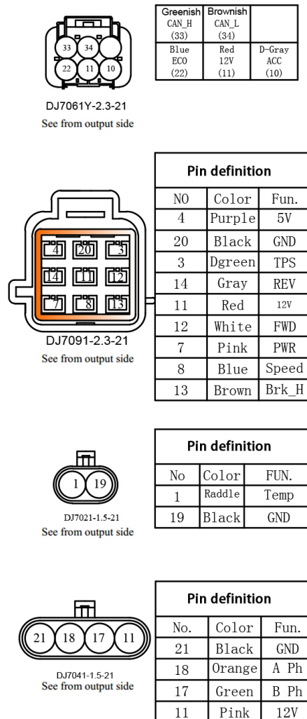
Figure 8: Definition for each I/O port
